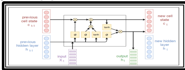
Figure 3. LSTM architecture [22]
