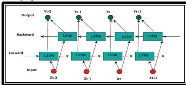
Figure 4. BI-LSTM architecture [23]
